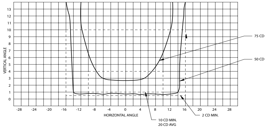
FAA L-852A Narrow (Straight Section), CAT II
